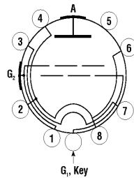
4X150A/7034 Connection Diagram
