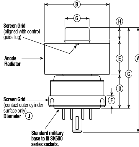
4X150A/7034 Outline Drawing
