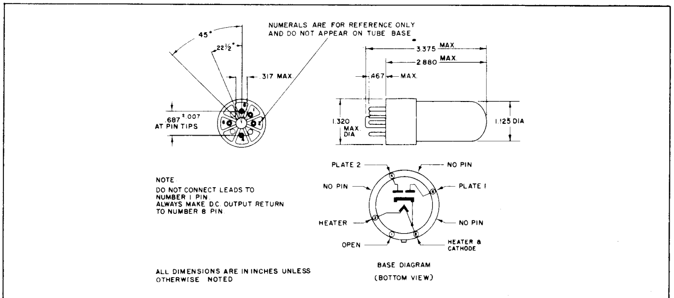
OUTLINE DRAWING
