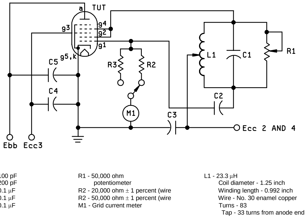
FIGURE 1237-1. Converter tube test oscillator circuit.
