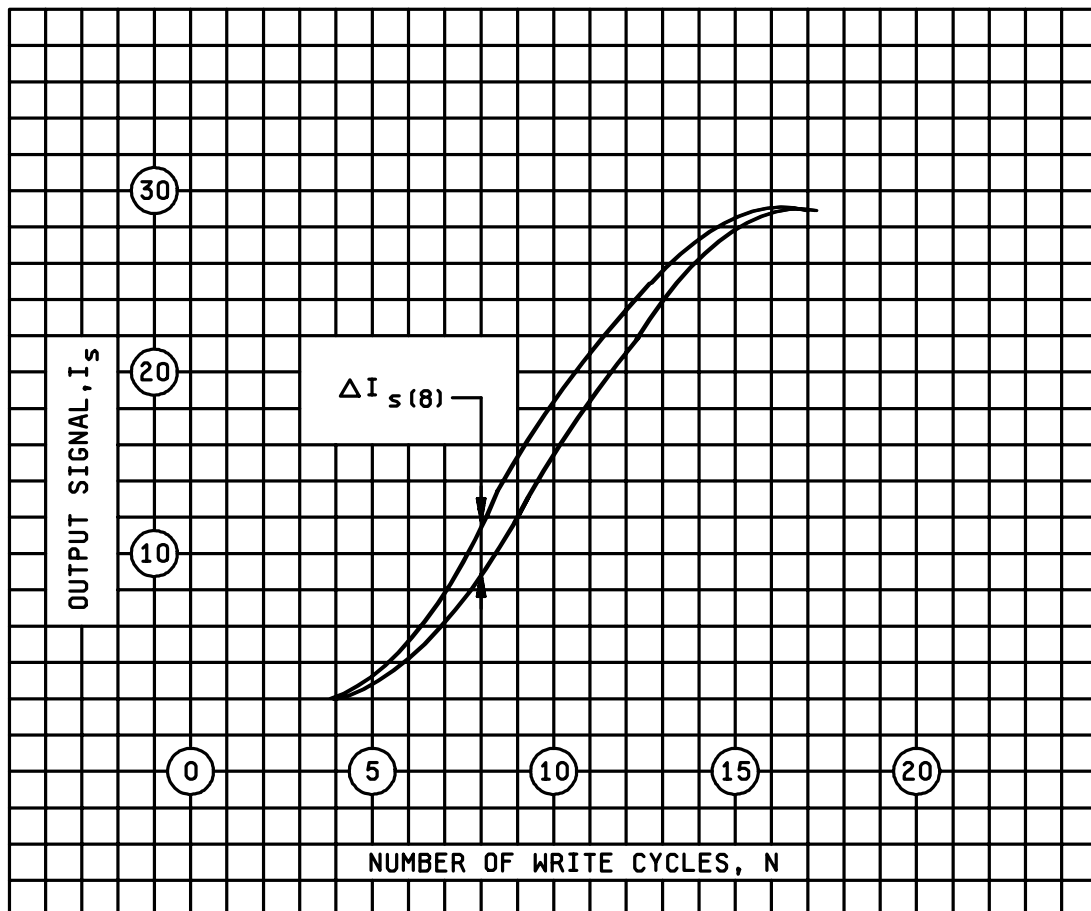
FIGURE 5424-2. Output levels plotted from oscilloscope data.
