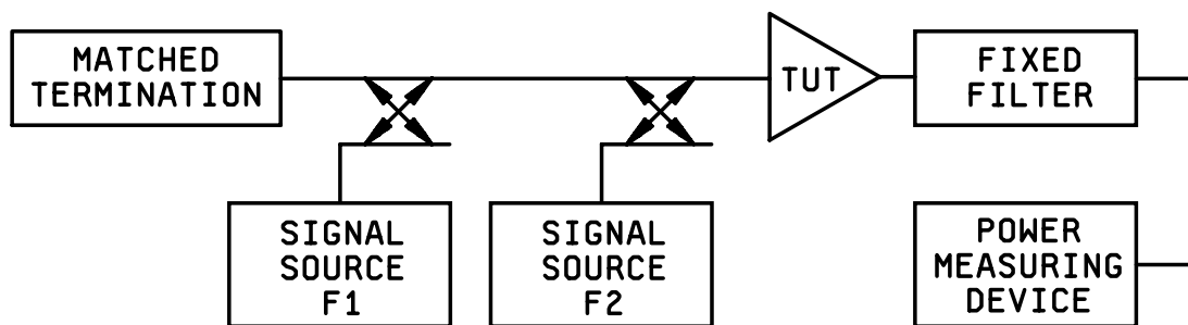
FIGURE 4263-2. Cross modulation.
