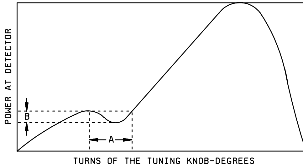
FIGURE 4426-2. Tuning characteristics.
