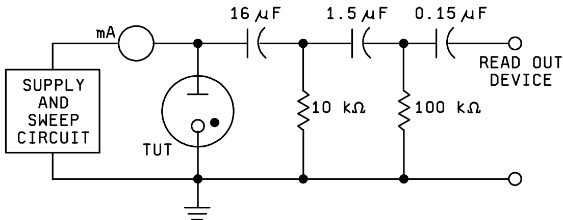
FIGURE 3345-1. Test circuit.
