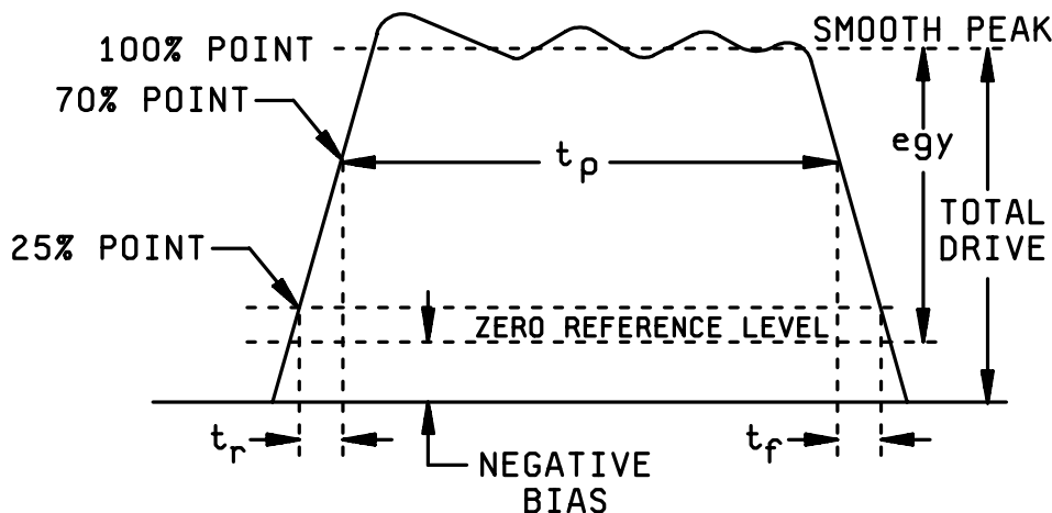
FIGURE 3. Grid pulse.
