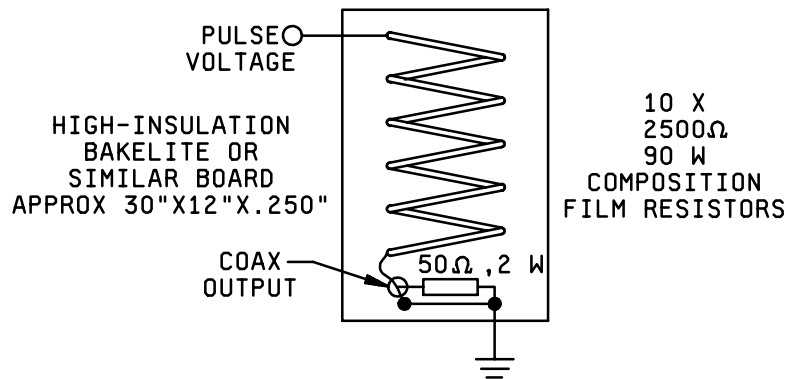
FIGURE 4306-4. Resistive divider.
