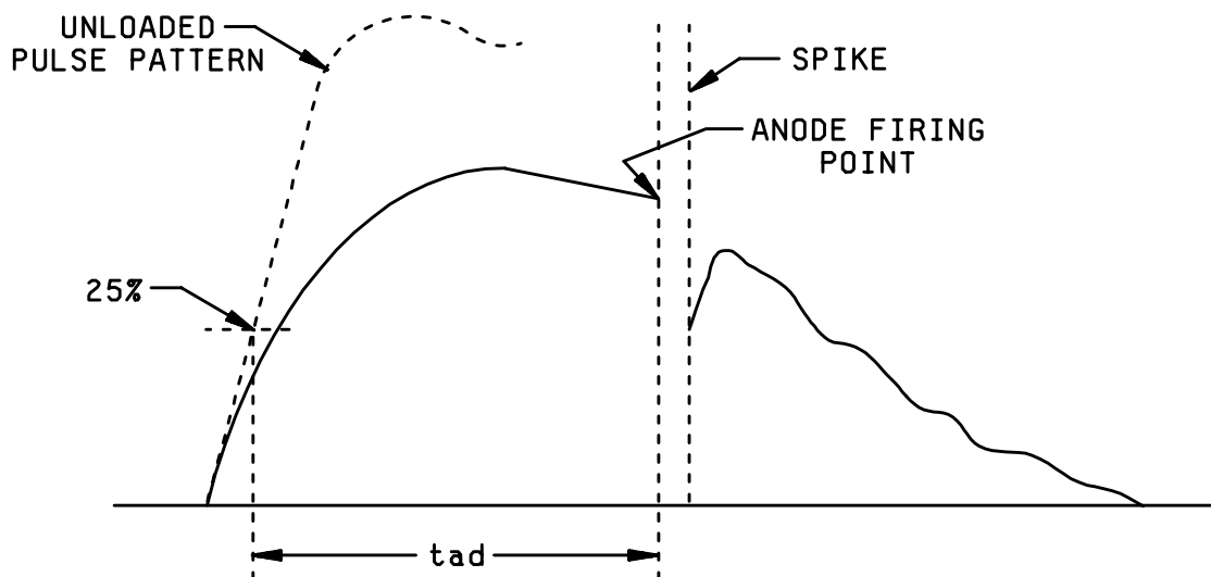
FIGURE 3256-1. Grid pulse (anode conducting) .
