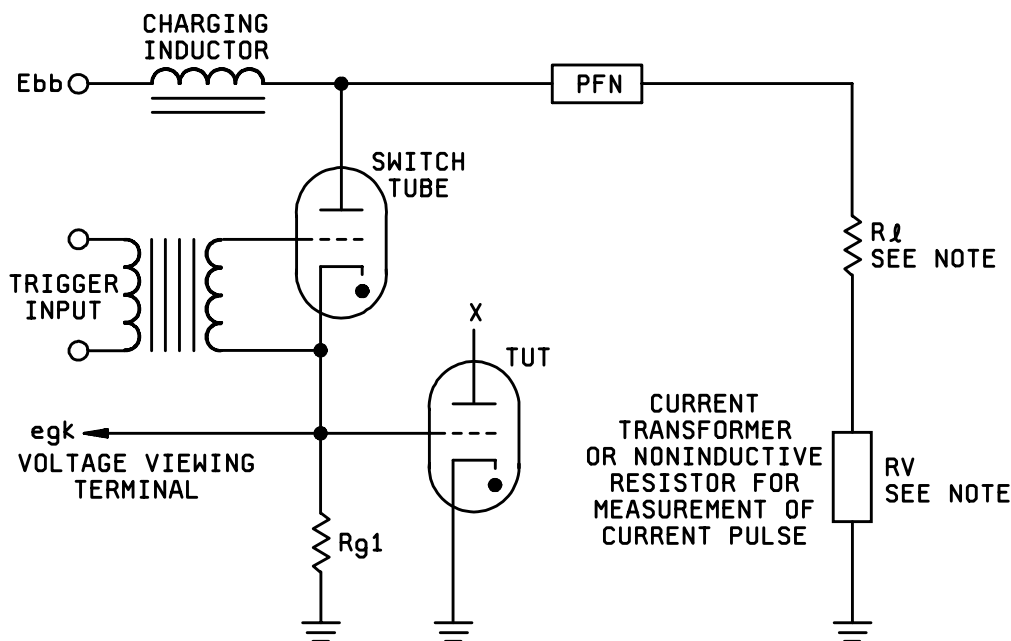
FIGURE 3251-1. Pulse emission test circuit.
