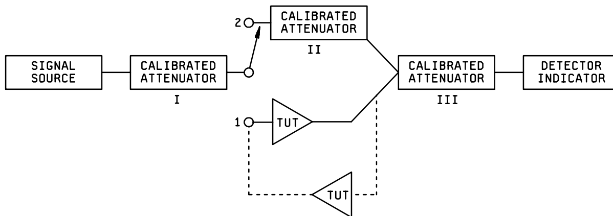
FIGURE 4257-1. Substitution method .
