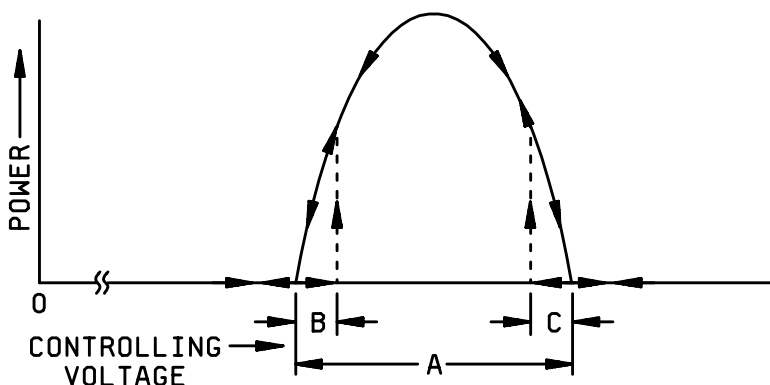
FIGURE 4231-1. Hysteresis (1).
