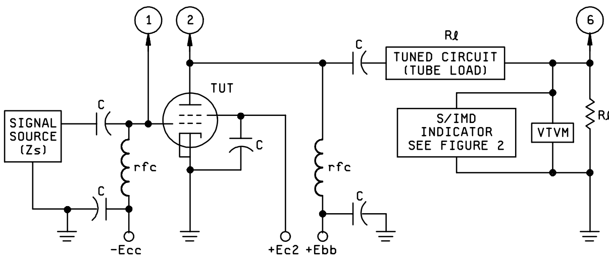
FIGURE 2206-2. S/IMD measurement.
