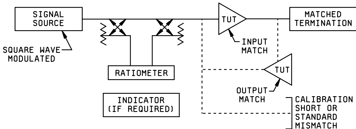
FIGURE 4256-1. Reflectometer method.
