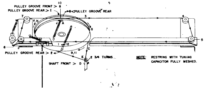
Fig. 7. Dial cable stringing procedure
